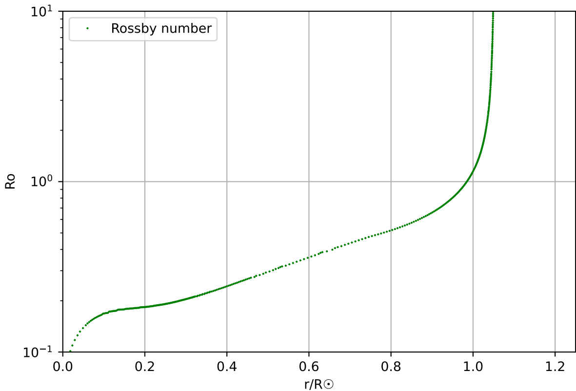
Rossby number, profile 154, age 6.22 \times 10^9
